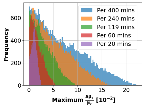
Figure 10: Maximum change in \Delta \text{chrom } \beta_y/\beta_y for HL-LHCb1 flat optics over several different time intervals.
