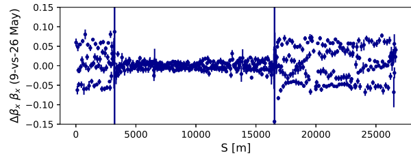
Figure 1: Measured relative optics shift for LHC beam 1 (LHCb1) between 9 and 26 May 2022 for same machine configuration at \beta^* 30 cm [1].
