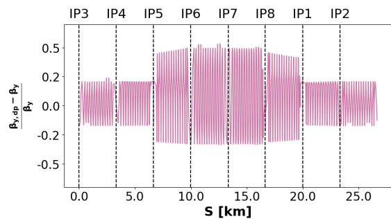
Figure 2: Vertical \beta -beating for HL-LHCb1 corresponding to an \Delta p/p offset of \approx 2 \times 10^{-4} using round optics.
