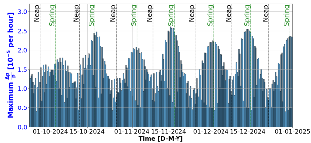
Figure 6: Maximum change in YASP-predicted \Delta p/p over an hour. Spring (green) and neap (black) tide times taken from [10].
