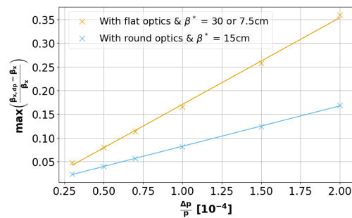
Figure 9: Predicted maximum \Delta \text{chrom } \beta_x/\beta_x for HL-LHCb1 as a function of \Delta p/p .
