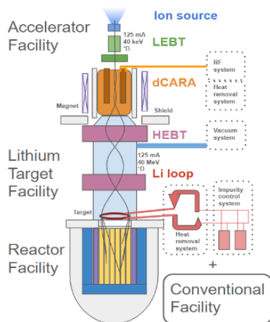
Figure 2: Conceptual configuration based on dCARA to produce neutrons for activation of a subcritical nuclear reactor and transmutation of waste nuclear fuel, including dCARA, low energy beam transport (LEBT), high energy beam transport (HEBT), and integrated neutron breakup target, with a footprint similar to a small modular reactor (SMR).
