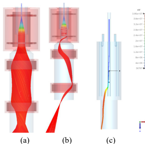
Figure 1: (a) Superposition of deuteron orbits in dCARA with deuteron injected at all RF phases, indicating beam envelope; (b) deuteron orbit injected at one given RF phase using CST Tracking solver; and (c) instantaneous spatial distribution of deuteron beam in dCARA using CST PIC solver. The main magnet and HEBT magnets are shown as red shells.
