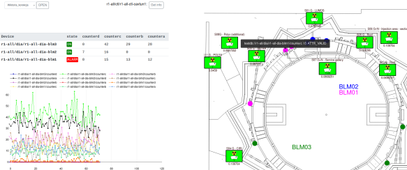
Figure 2: Beam Loss Monitoring GUI displaying radiation monitoring stations (green squares) and Beam Loss Detector locations (purple, blue, and dark green dots) overlaid on the machine layout.
