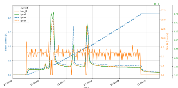
Figure 3: Beam loss during the injection procedure. The accumulated beam current (blue) stops increasing as vacuum pressure rises in the gun section (green), while the BLD counter signal (orange) reflects the presence or absence of beam loss events.
