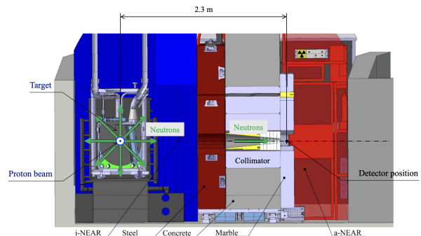
Figure 1: Model of the n_TOF spallation target with the neighboring measurement station for neutron activation measurements, the so-called "a-NEAR", where diamond dosimeters were installed to measure the fast neutron beam.
