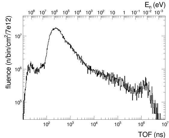
Figure 2: Neutron fluence at a-NEAR as function of time-of-flight. Neutrons with E_n > 3 \text{ MeV} arrive in the first 100 ns at the detector position.
